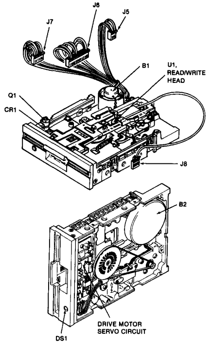
Fig. A-21. Drive unit parts layout, Model 1541.
